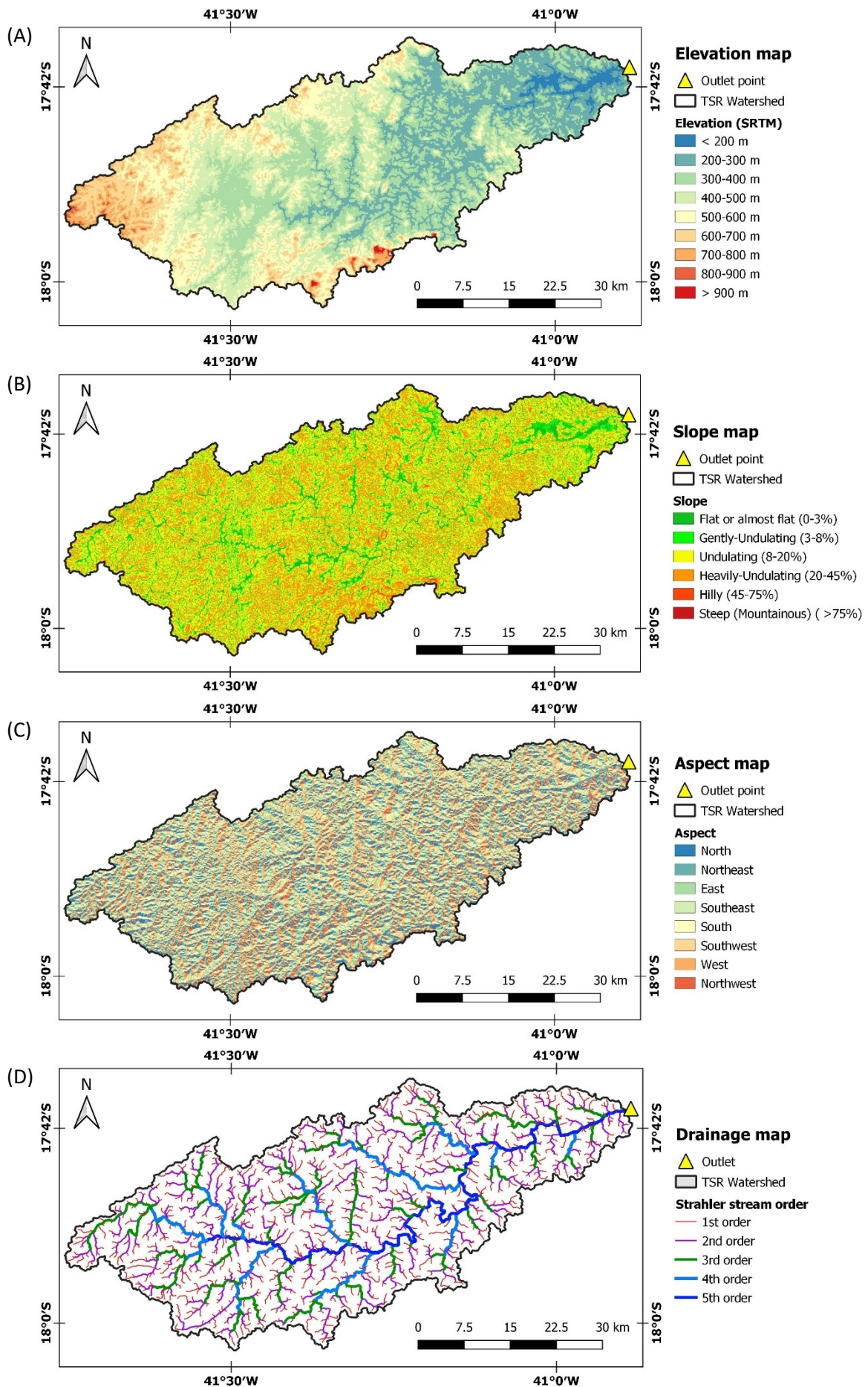
Figure 5 – Morphometric and drainage maps of the Todos Santos River Basin. (A) Elevation map with reclassified SRTM data. (B) Slope map according to the Embrapa relief classes. (C) Aspect map with direction orientation. (D). Drainage map with stream orders.
