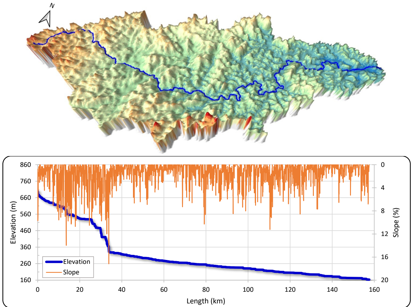
Figure 6 – 3D view of the watershed of the Todos os Santos River, the blue line indicates the main course of the river (top panel). The graph illustrating the behavior of slope and elevation along the Todos os Santos River (bottom panel).
